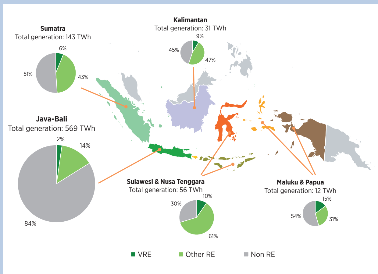
Figure 19: On-grid power generation in the Reference Case for 2030
