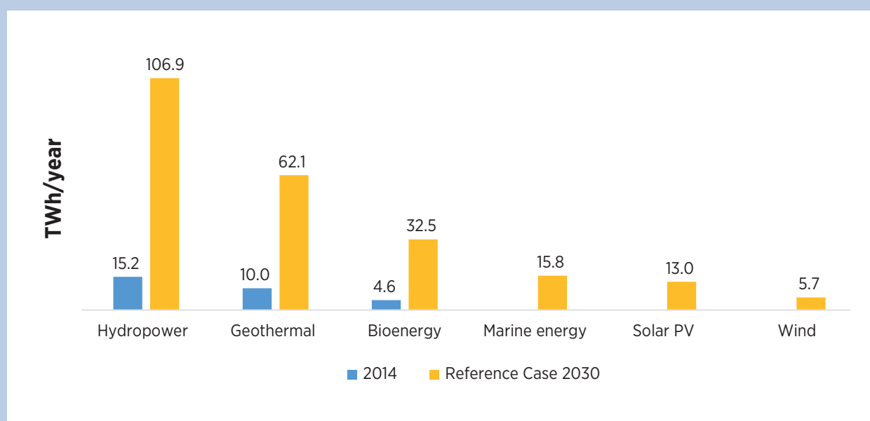
Figure 20: Renewable power generation in Indonesia, 2014 and in the Reference Case for 2030
