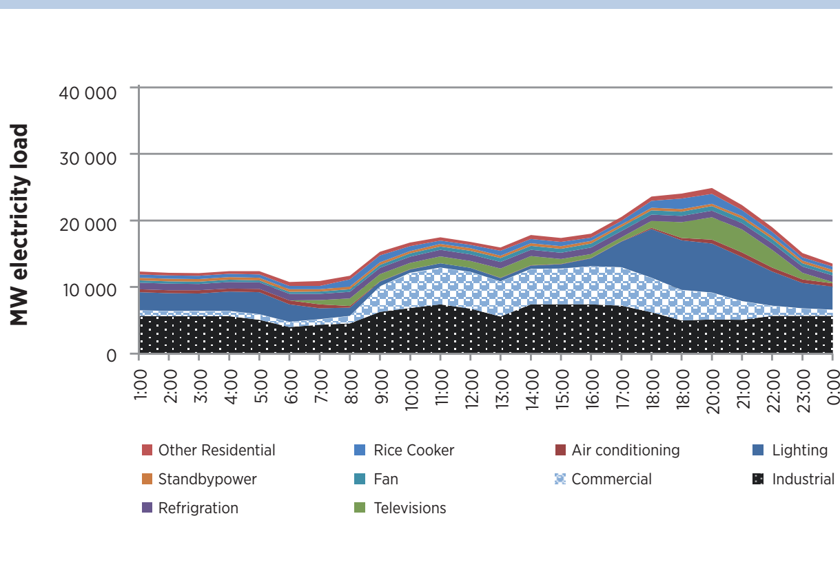
Figure 23: Modelled daily electricity demand in Indonesia in 2010
