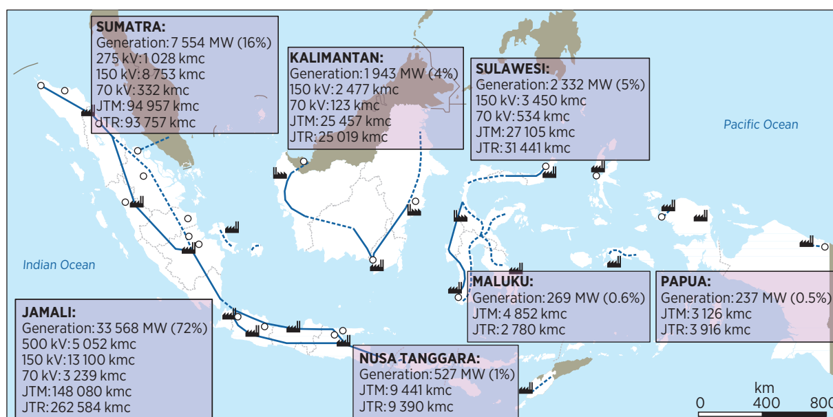
Figure 13: Electricity network in Indonesia, 2014
