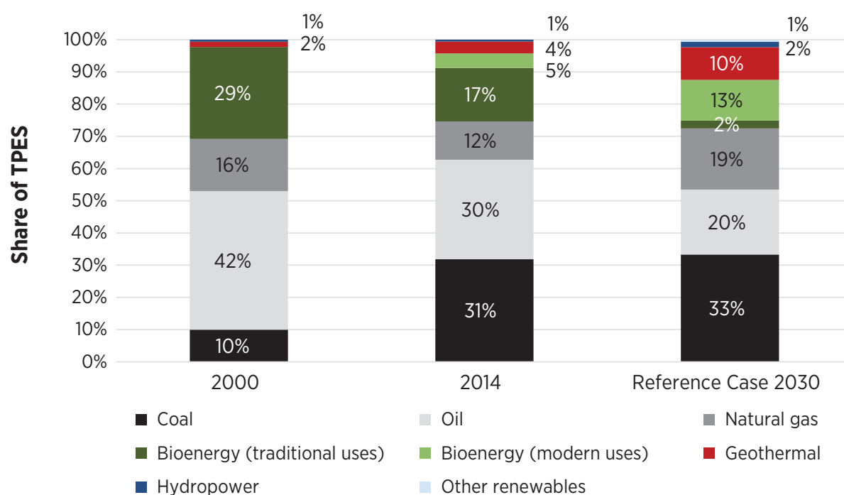
Figure 16: Fuel mix in primary energy supply, 2000, 2014 and in the Reference Case for 2030
