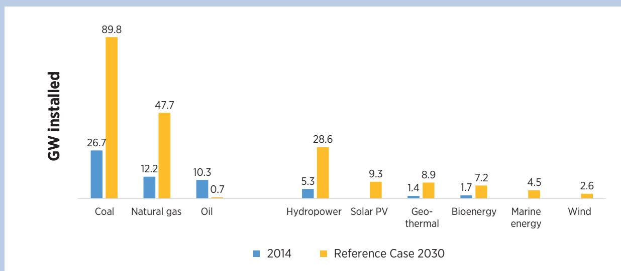
Figure 21: Total installed power generation capacity in Indonesia, 2014 and in the Reference Case for 2030
